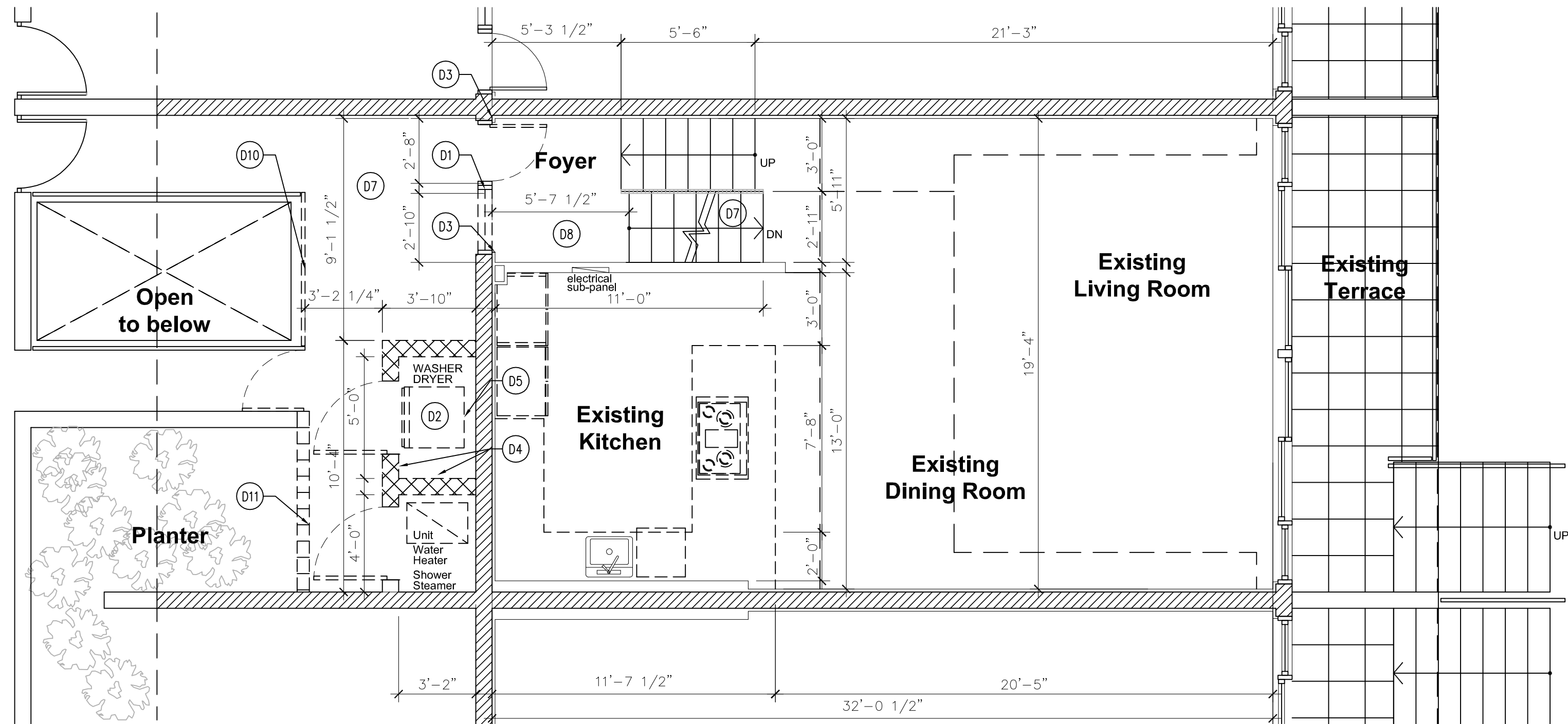
DEMOLITION: 2ND FLOOR PLAN 1/4"= 1'-0"
