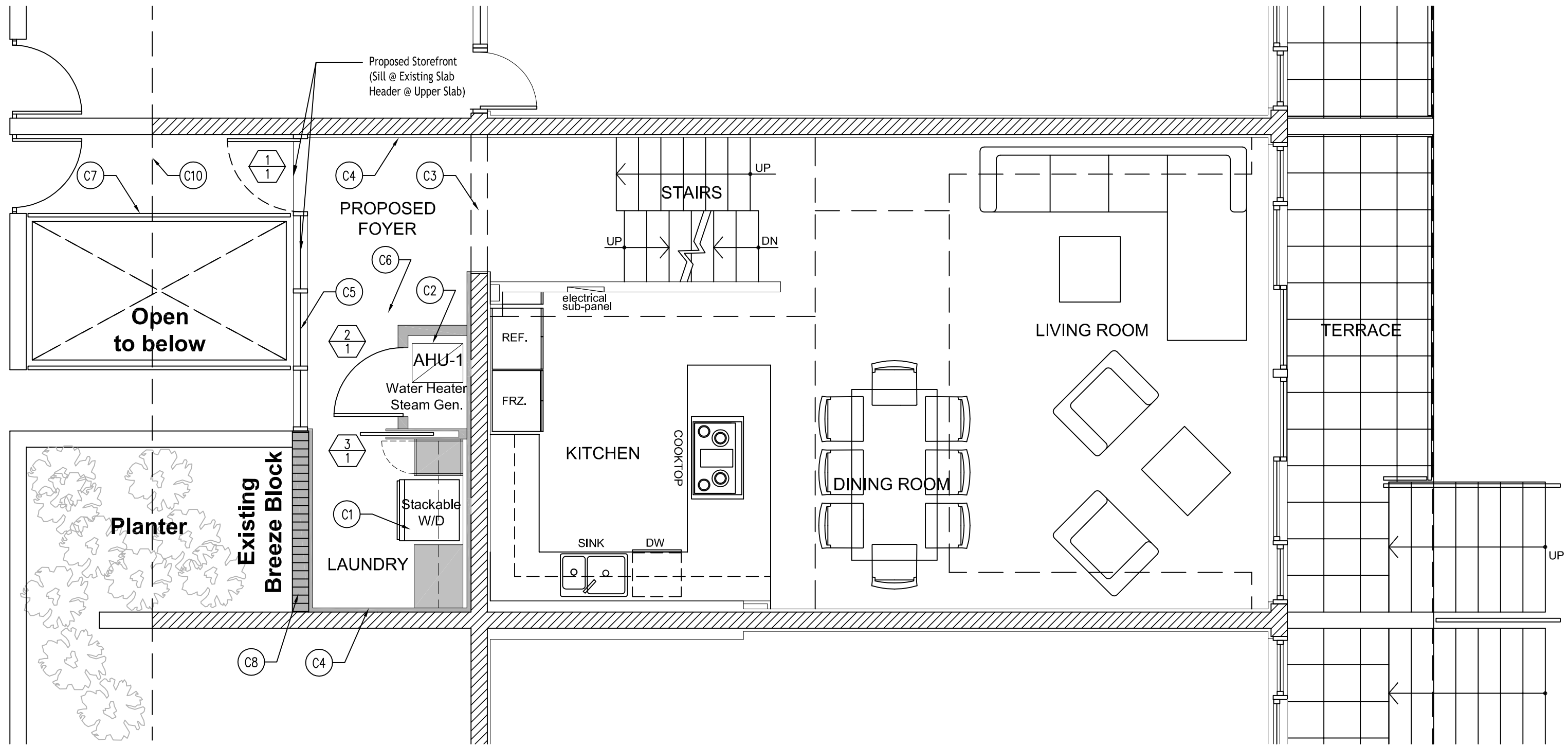
PROPOSED: 2ND FLOOR PLAN 1/4"= 1'-0" Proposed Additional S.F. = 129 s.f.
